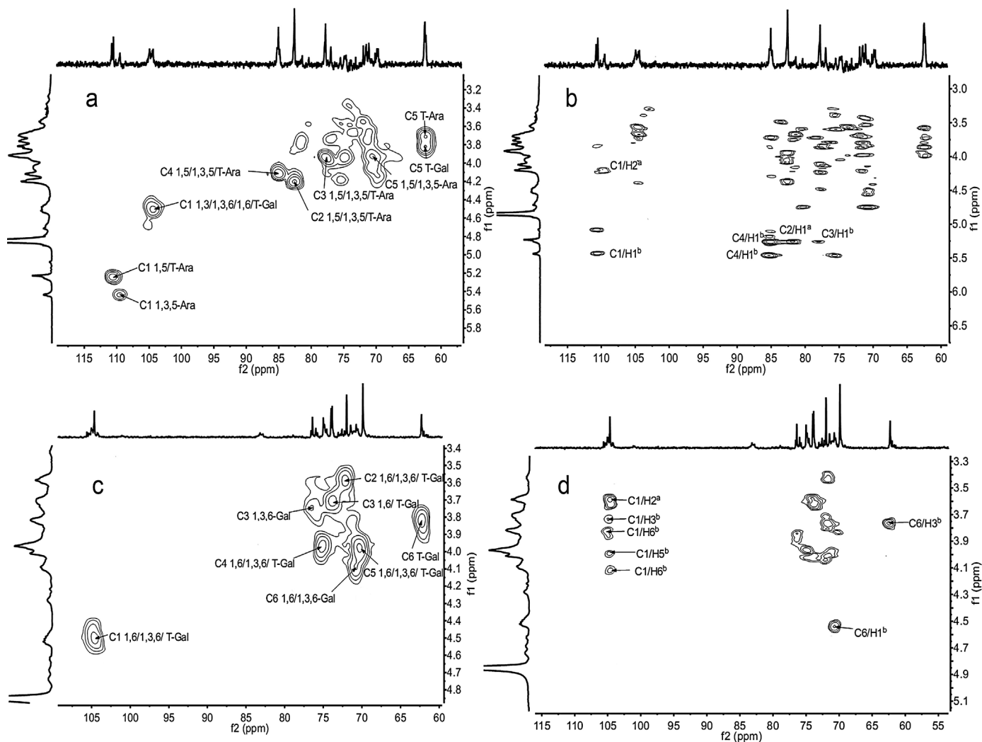
Fig. 2. ^2\text{D} NMR spectra of RN1 and RN1N2. (a) HSQC spectrum of RN1; (b) HMBC spectrum of RN1; (c) HSQC spectrum of RN1N2; (d) HMBC spectrum of RN1N2. “a” means “intra-annular correlation” and “b” means “hetero-ring correlation” in (b and d).
